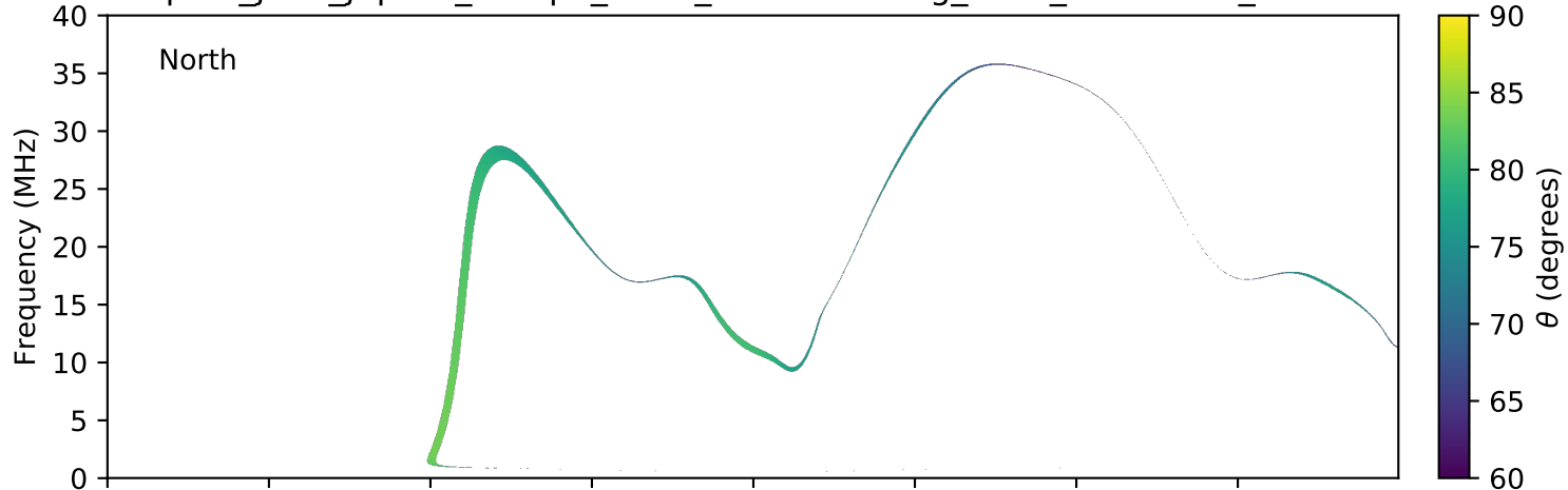
expres_juno_jupiter_europa_isaac_lossc-wid1deg_3kev_20161124_v01.cdf
