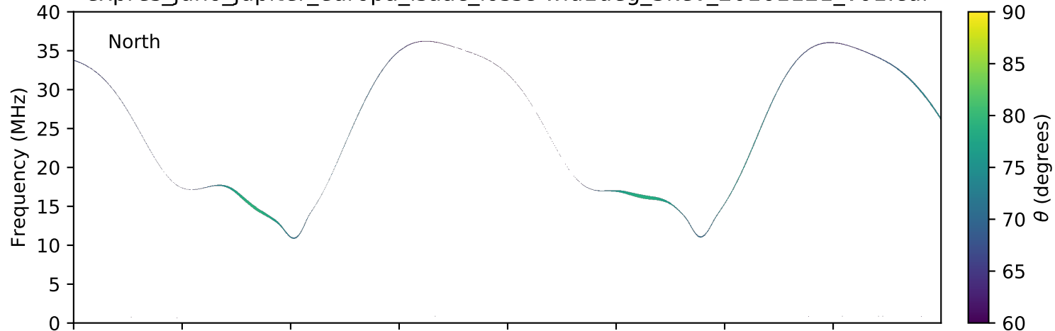
expres_juno_jupiter_europa_isaac_lossc-wid1deg_3kev_20161121_v01.cdf
