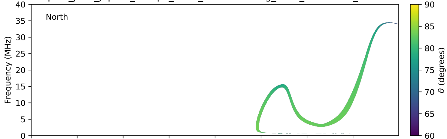
expres_juno_jupiter_europa_isaac_lossc-wid1deg_3kev_20161120_v01.cdf
