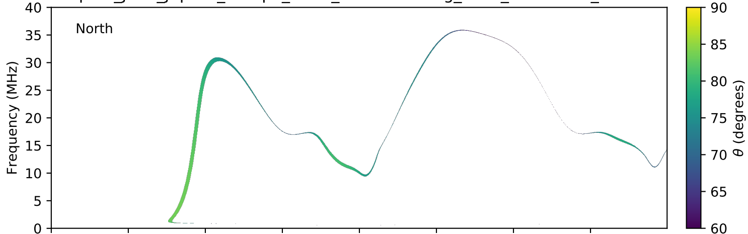
expres_juno_jupiter_europa_isaac_lossc-wid1deg_3kev_20161117_v01.cdf
