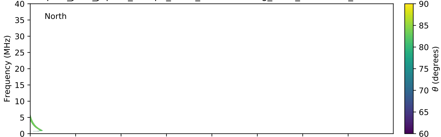
expres_juno_jupiter_europa_isaac_lossc-wid1deg_3kev_20161115_v01.cdf
