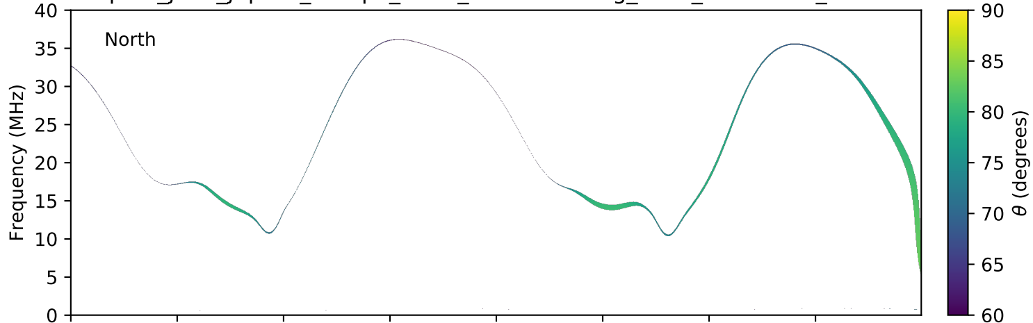
expres_juno_jupiter_europa_isaac_lossc-wid1deg_3kev_20161114_v01.cdf
