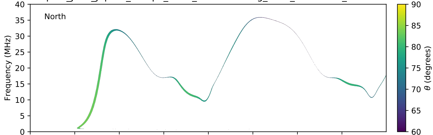
expres_juno_jupiter_europa_isaac_lossc-wid1deg_3kev_20161110_v01.cdf
