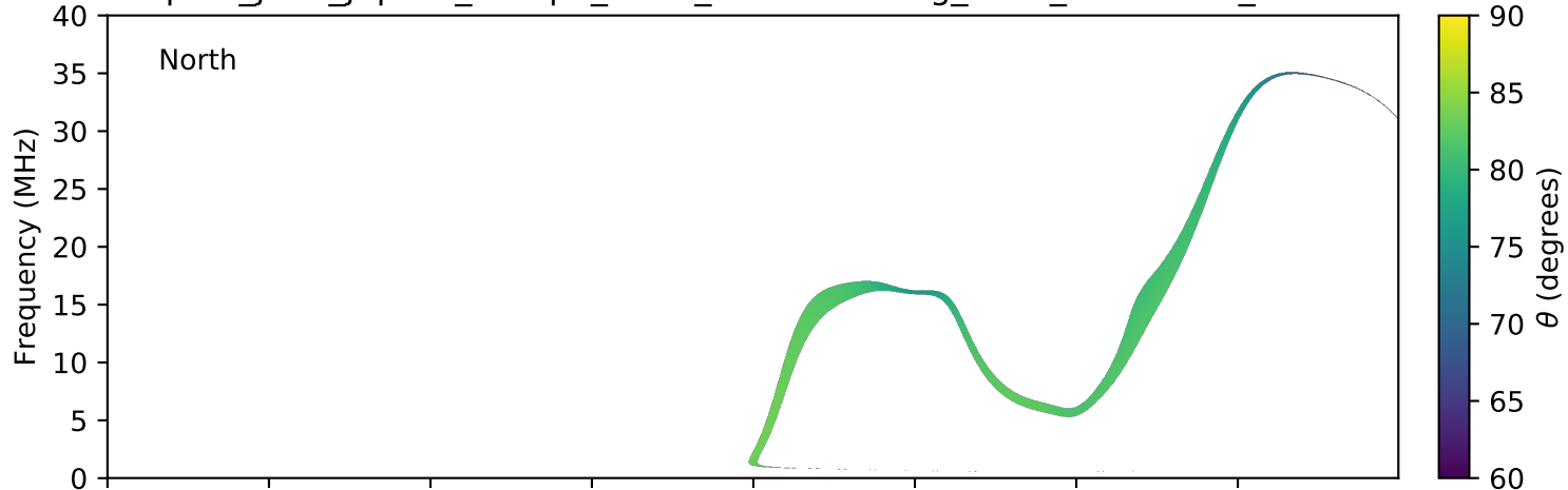
expres_juno_jupiter_europa_isaac_lossc-wid1deg_3kev_20161106_v01.cdf
