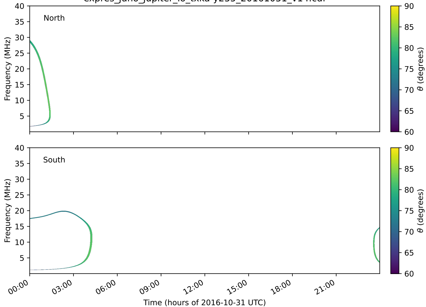
expres_juno_jupiter_io_txka-y235_20161031_v14.cdf
