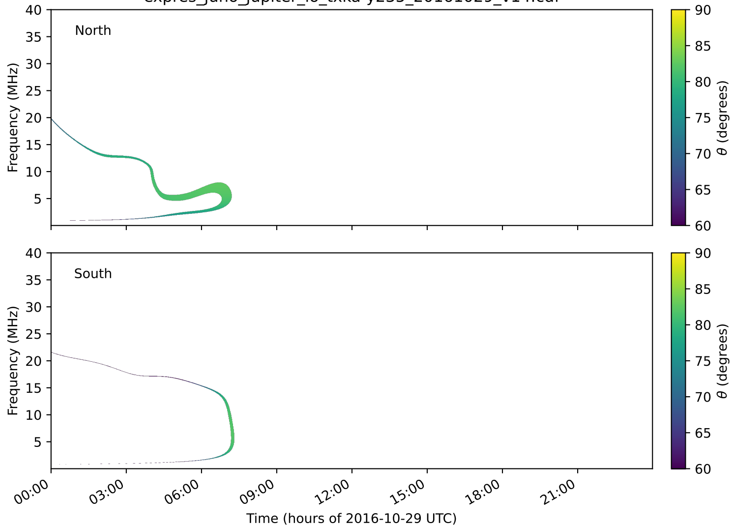
expres_juno_jupiter_io_txka-y235_20161029_v14.cdf
