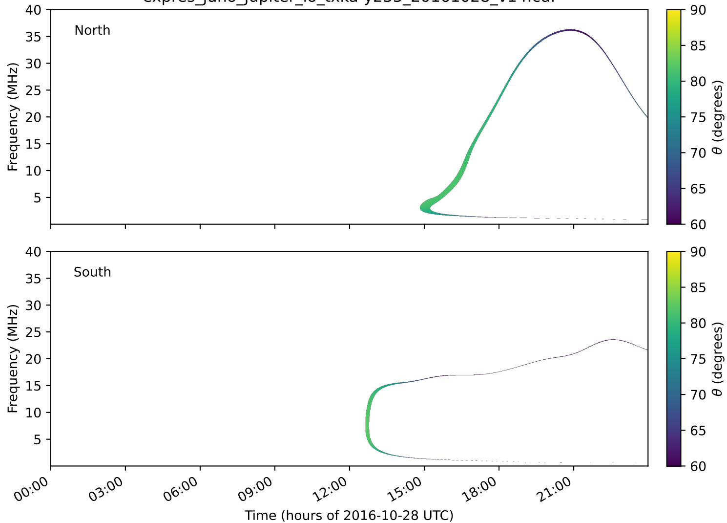
expres_juno_jupiter_io_txka-y235_20161028_v14.cdf
