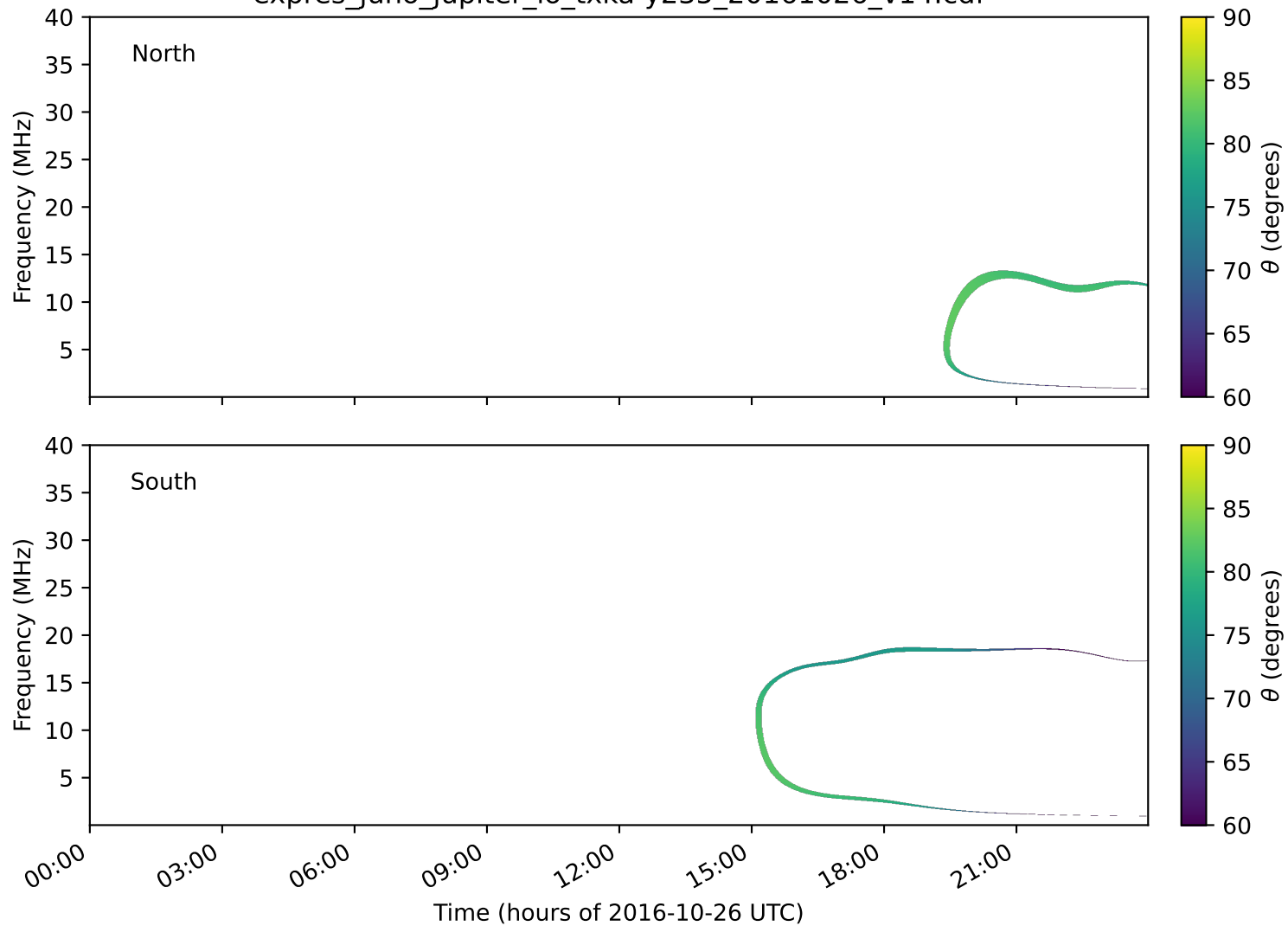
expres_juno_jupiter_io_txka-y235_20161026_v14.cdf
