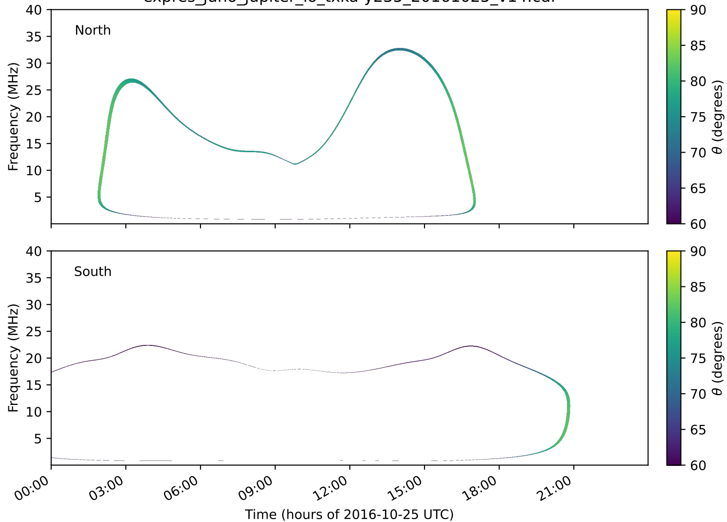
expres_juno_jupiter_io_txka-y235_20161025_v14.cdf
