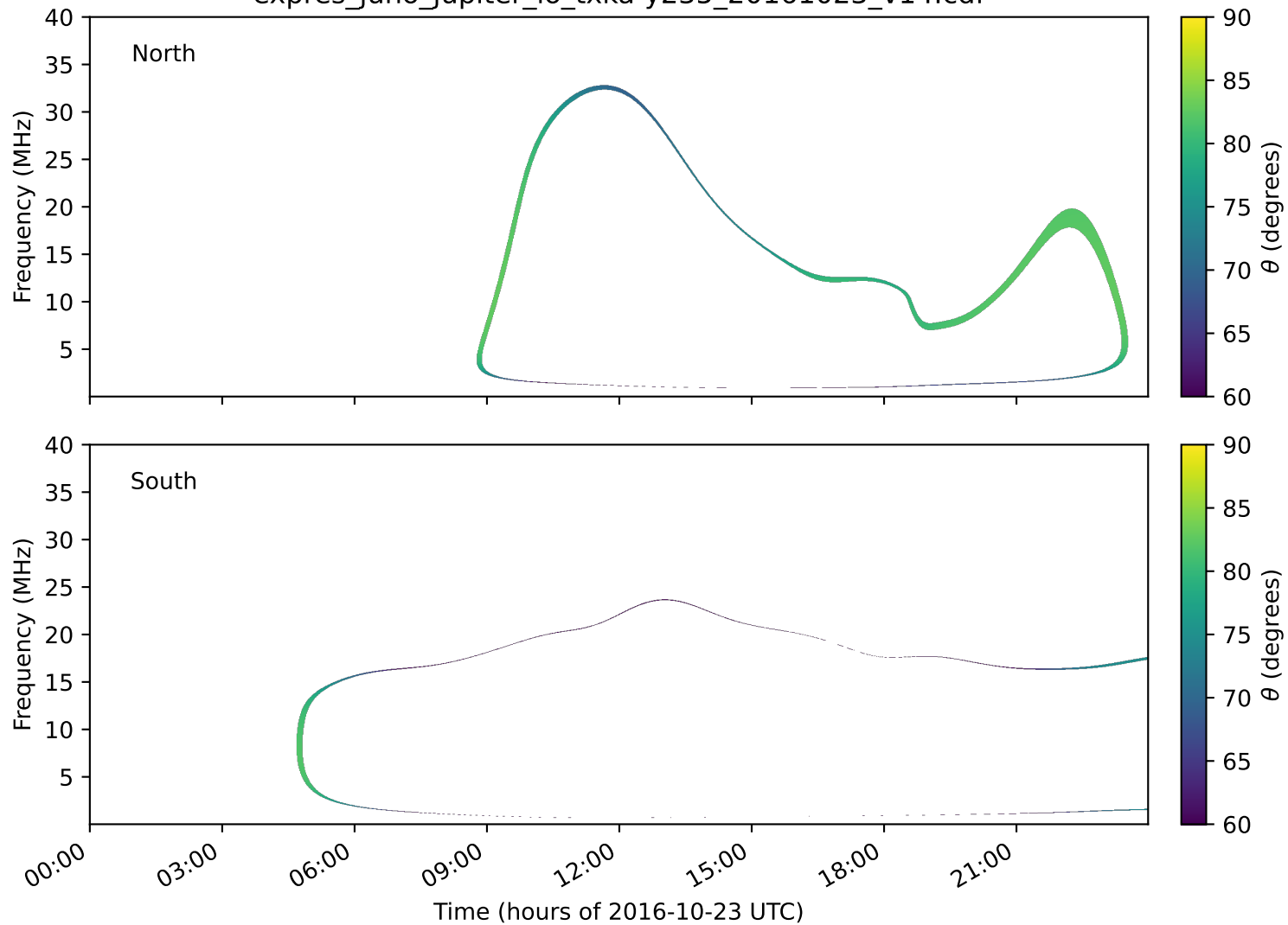
expres_juno_jupiter_io_txka-y235_20161023_v14.cdf
