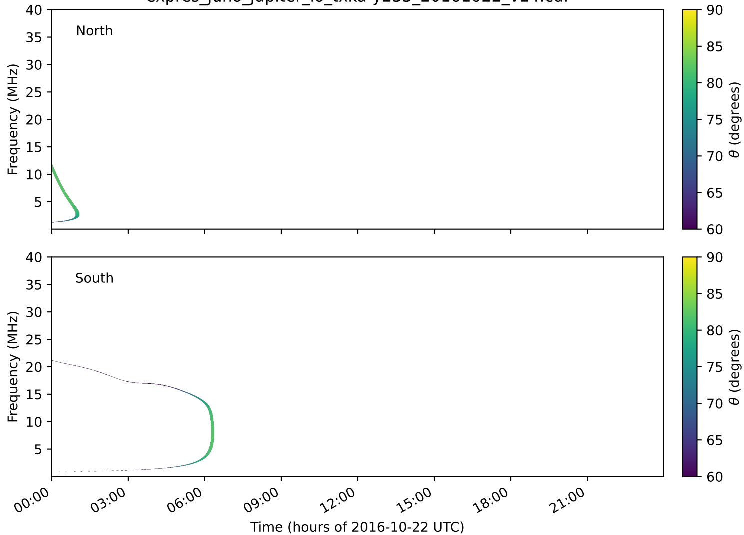
expres_juno_jupiter_io_txka-y235_20161022_v14.cdf
