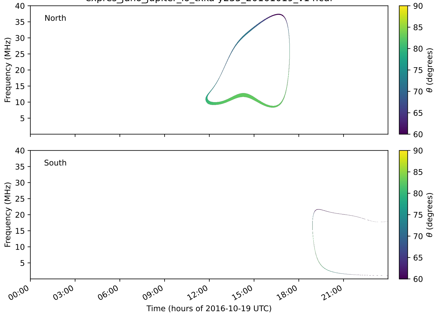
expres_juno_jupiter_io_txka-y235_20161019_v14.cdf
