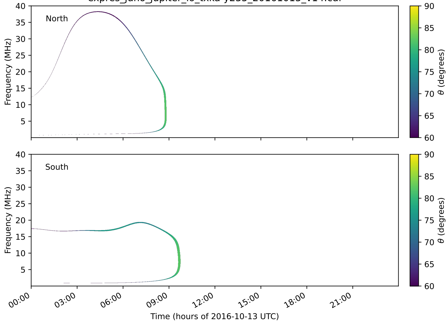
expres_juno_jupiter_io_txka-y235_20161013_v14.cdf
