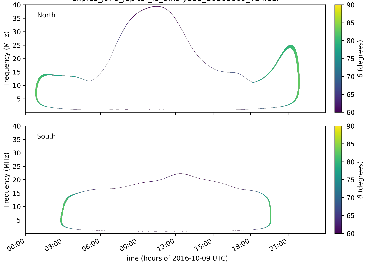
expres_juno_jupiter_io_txka-y235_20161009_v14.cdf
