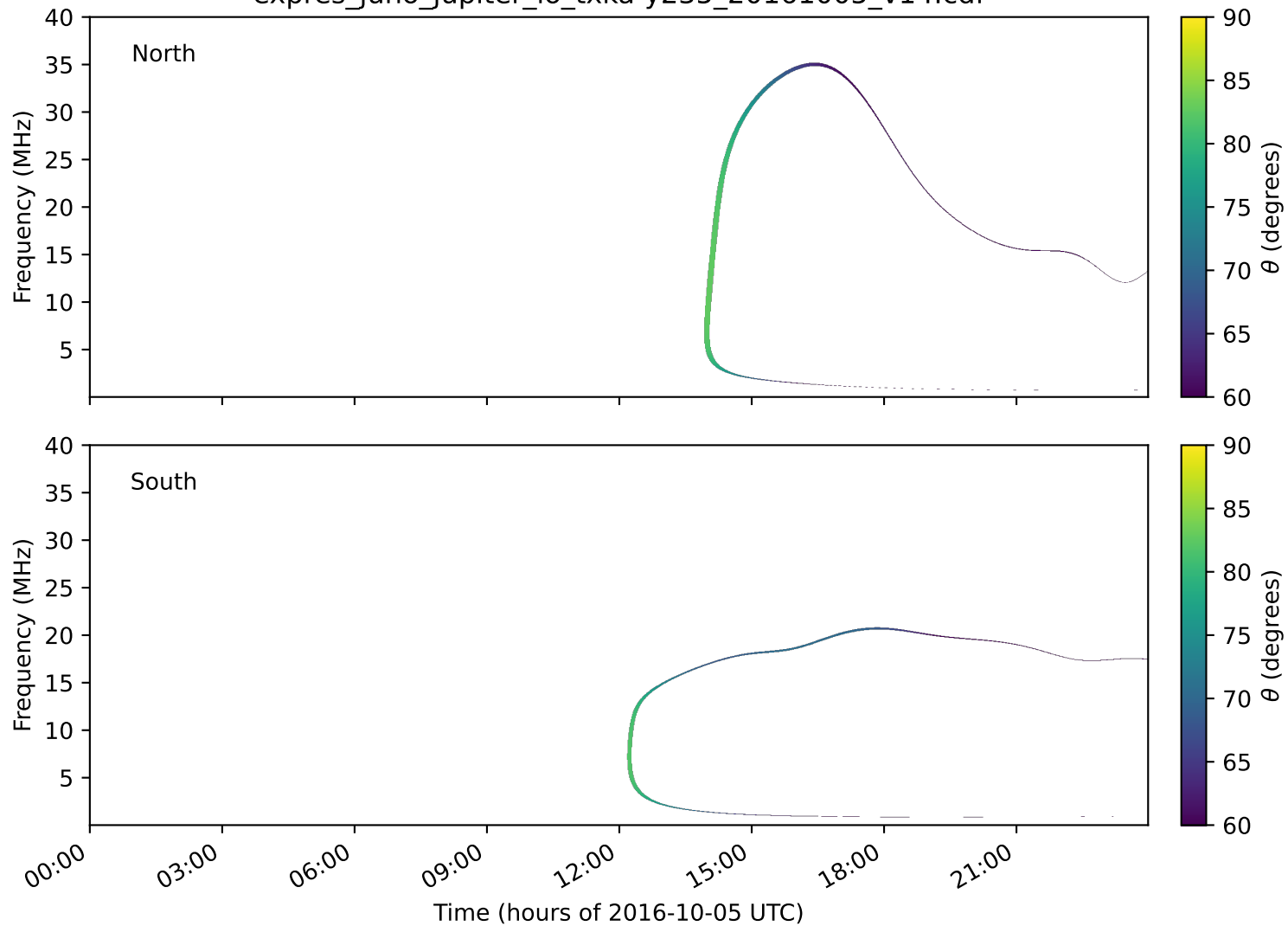
expres_juno_jupiter_io_txka-y235_20161005_v14.cdf
