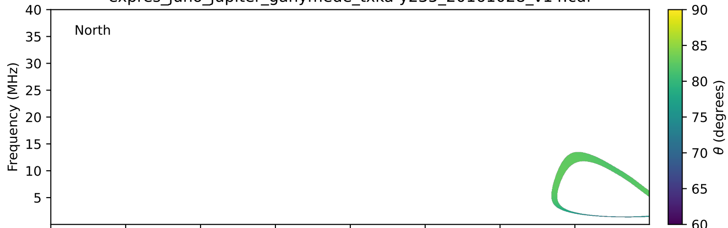
expres_juno_jupiter_ganymede_txka-y235_20161028_v14.cdf
