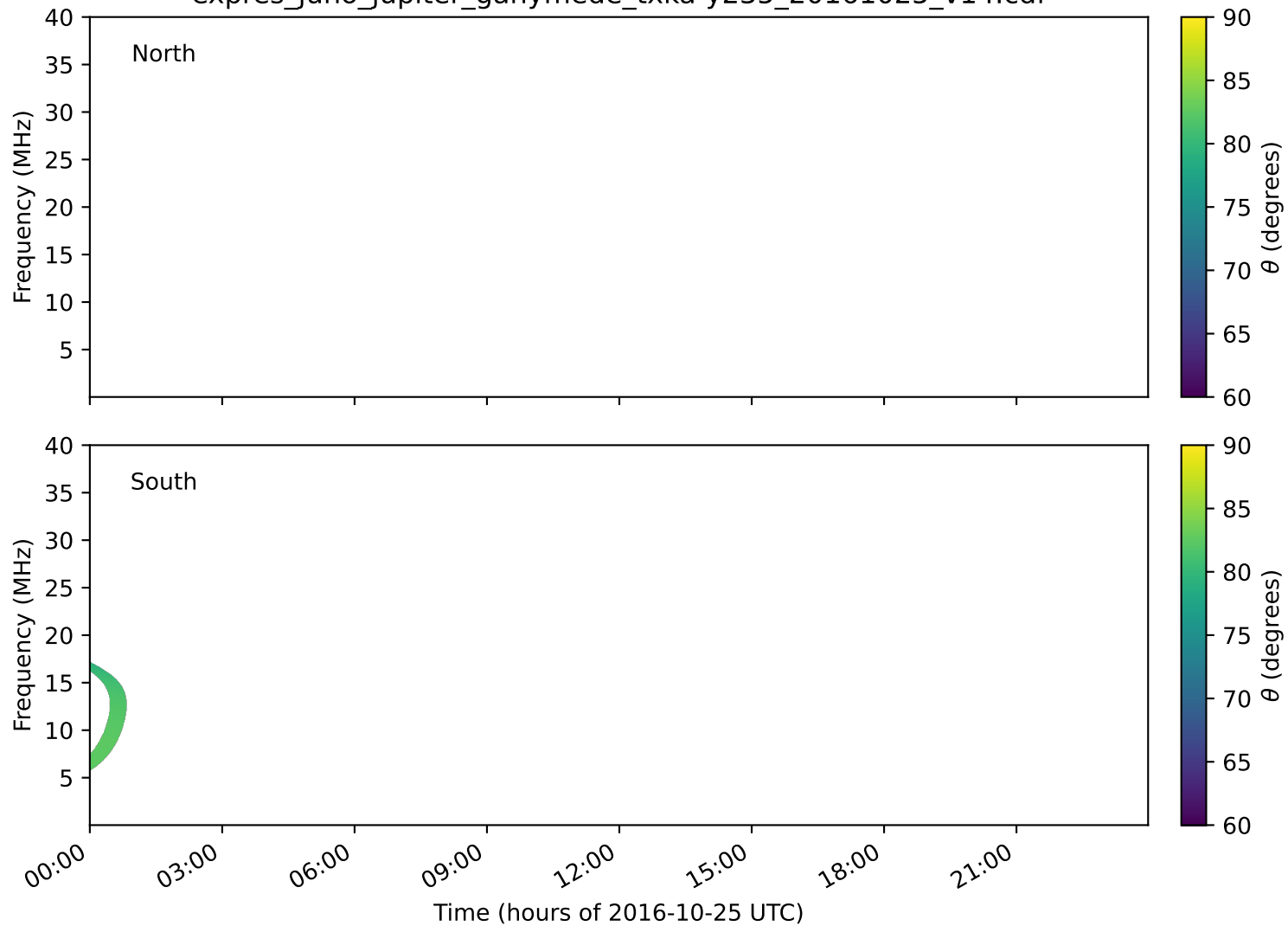
expres_juno_jupiter_ganymede_txka-y235_20161025_v14.cdf
