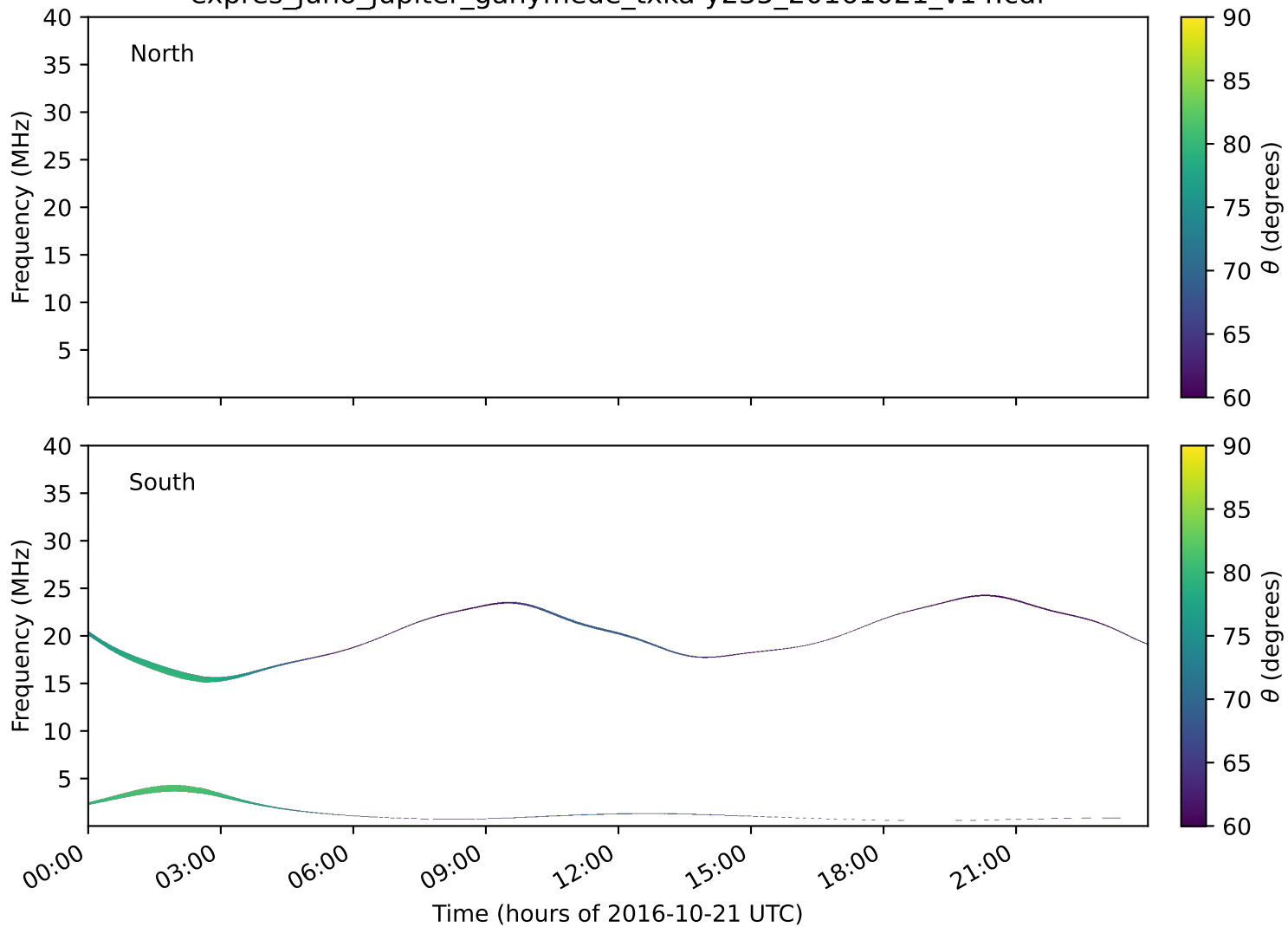
expres_juno_jupiter_ganymede_txka-y235_20161021_v14.cdf
