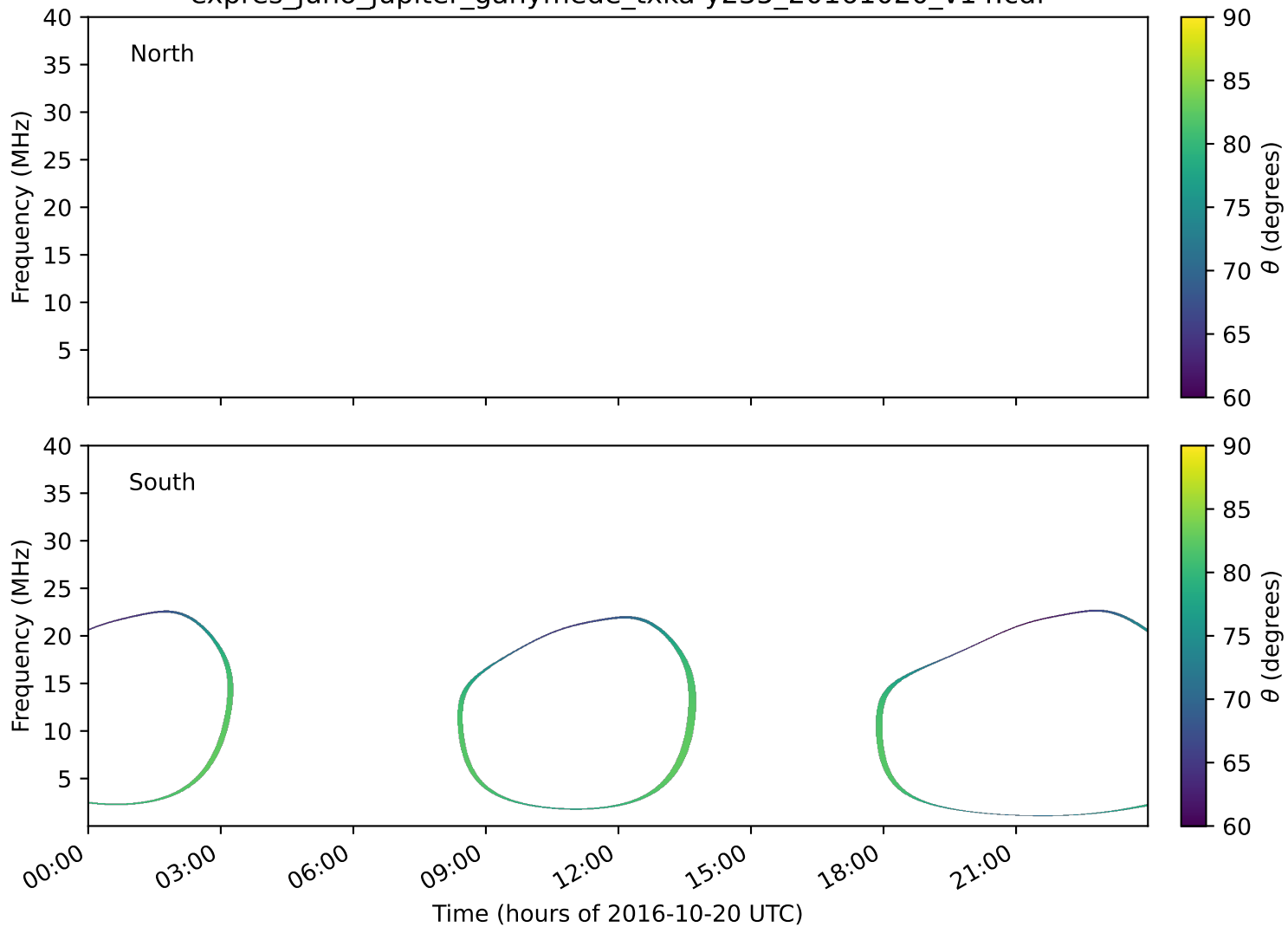
expres_juno_jupiter_ganymede_txka-y235_20161020_v14.cdf
