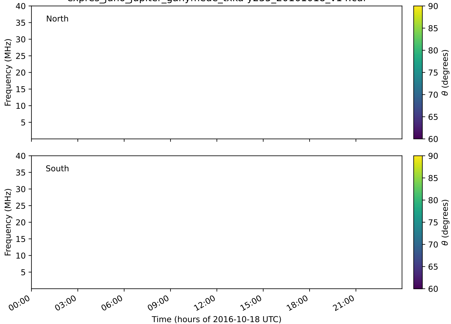
expres_juno_jupiter_ganymede_txka-y235_20161018_v14.cdf
