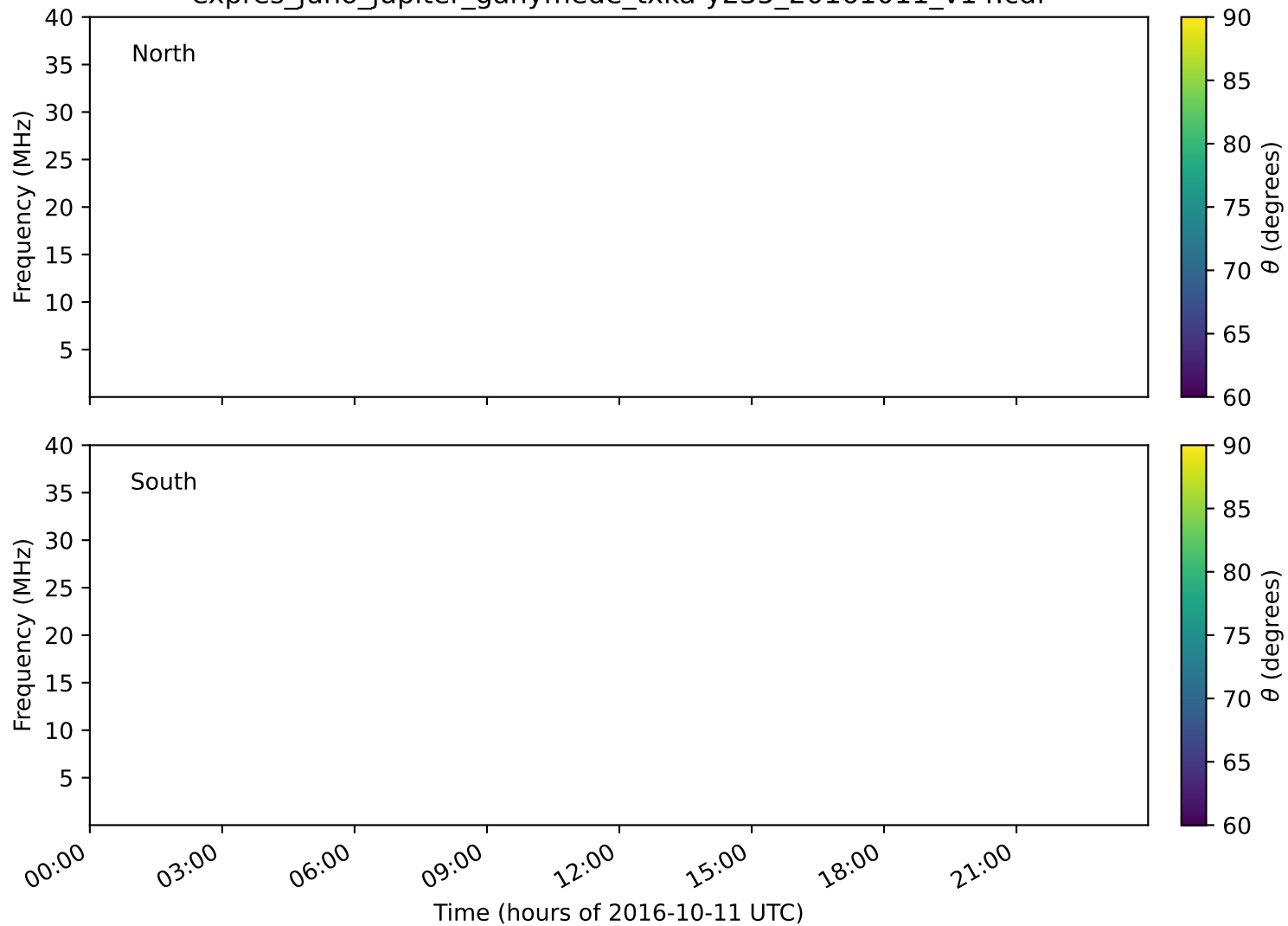
expres_juno_jupiter_ganymede_txka-y235_20161011_v14.cdf
