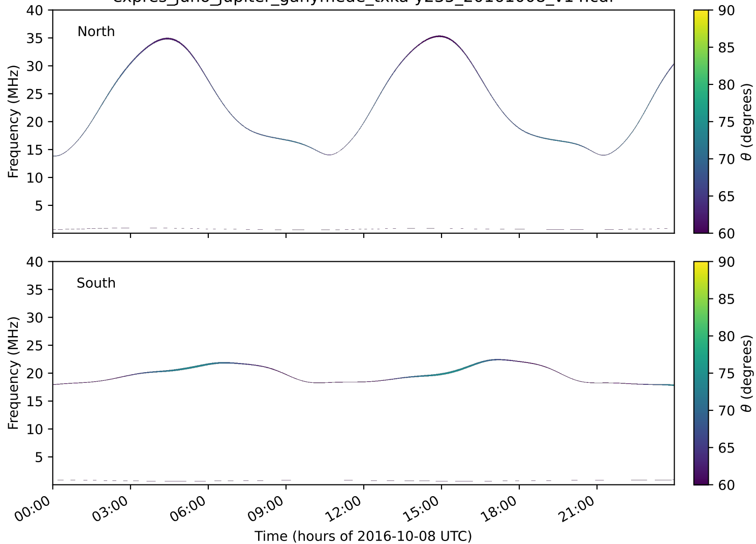
expres_juno_jupiter_ganymede_txka-y235_20161008_v14.cdf
