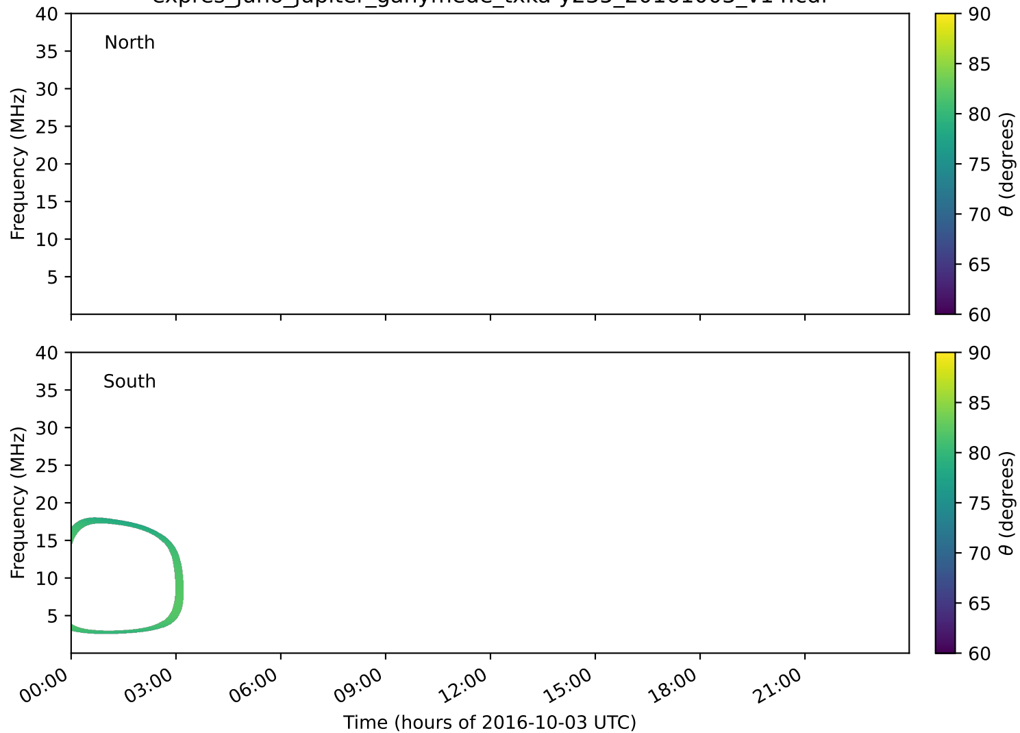
expres_juno_jupiter_ganymede_txka-y235_20161003_v14.cdf
