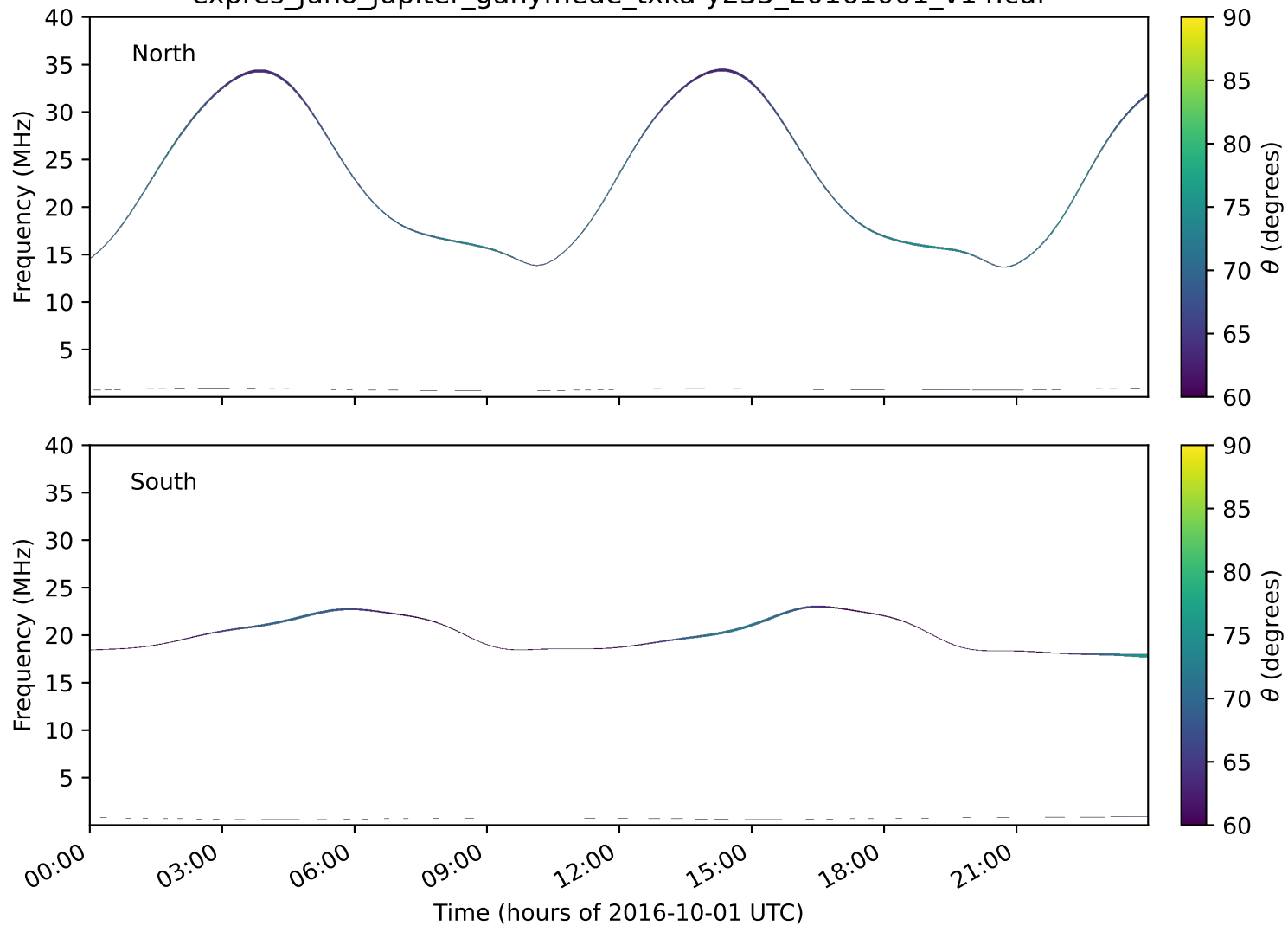
expres_juno_jupiter_ganymede_txka-y235_20161001_v14.cdf
