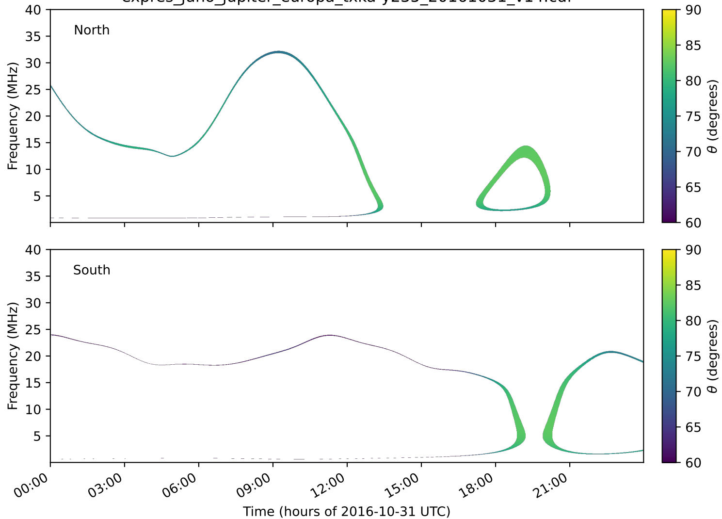
expres_juno_jupiter_europa_txka-y235_20161031_v14.cdf
