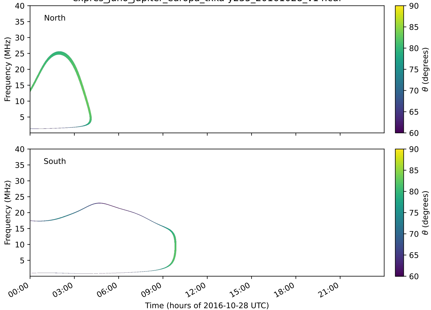
expres_juno_jupiter_europa_txka-y235_20161028_v14.cdf
