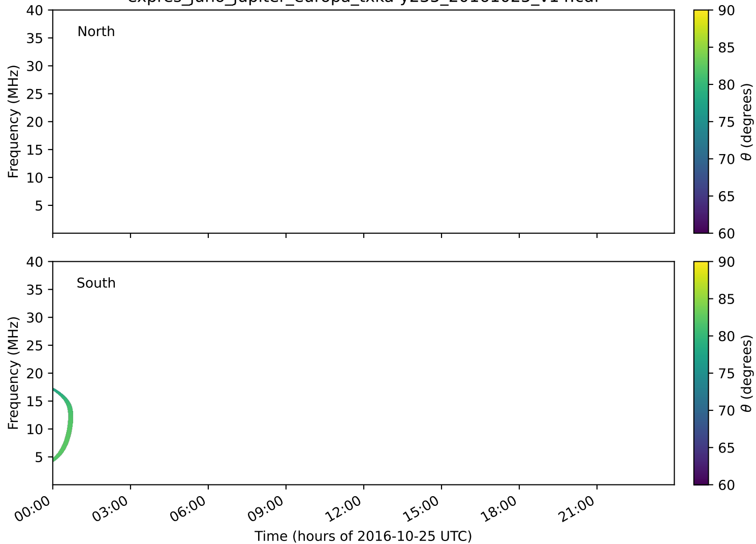
expres_juno_jupiter_europa_txka-y235_20161025_v14.cdf
