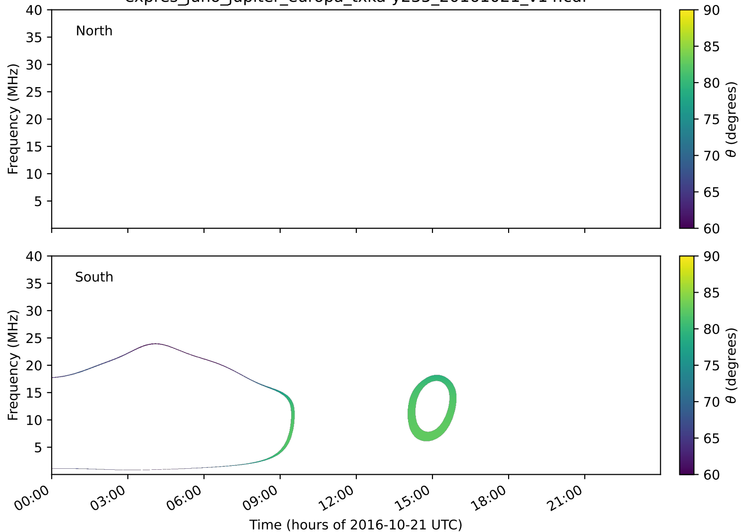
expres_juno_jupiter_europa_txka-y235_20161021_v14.cdf
