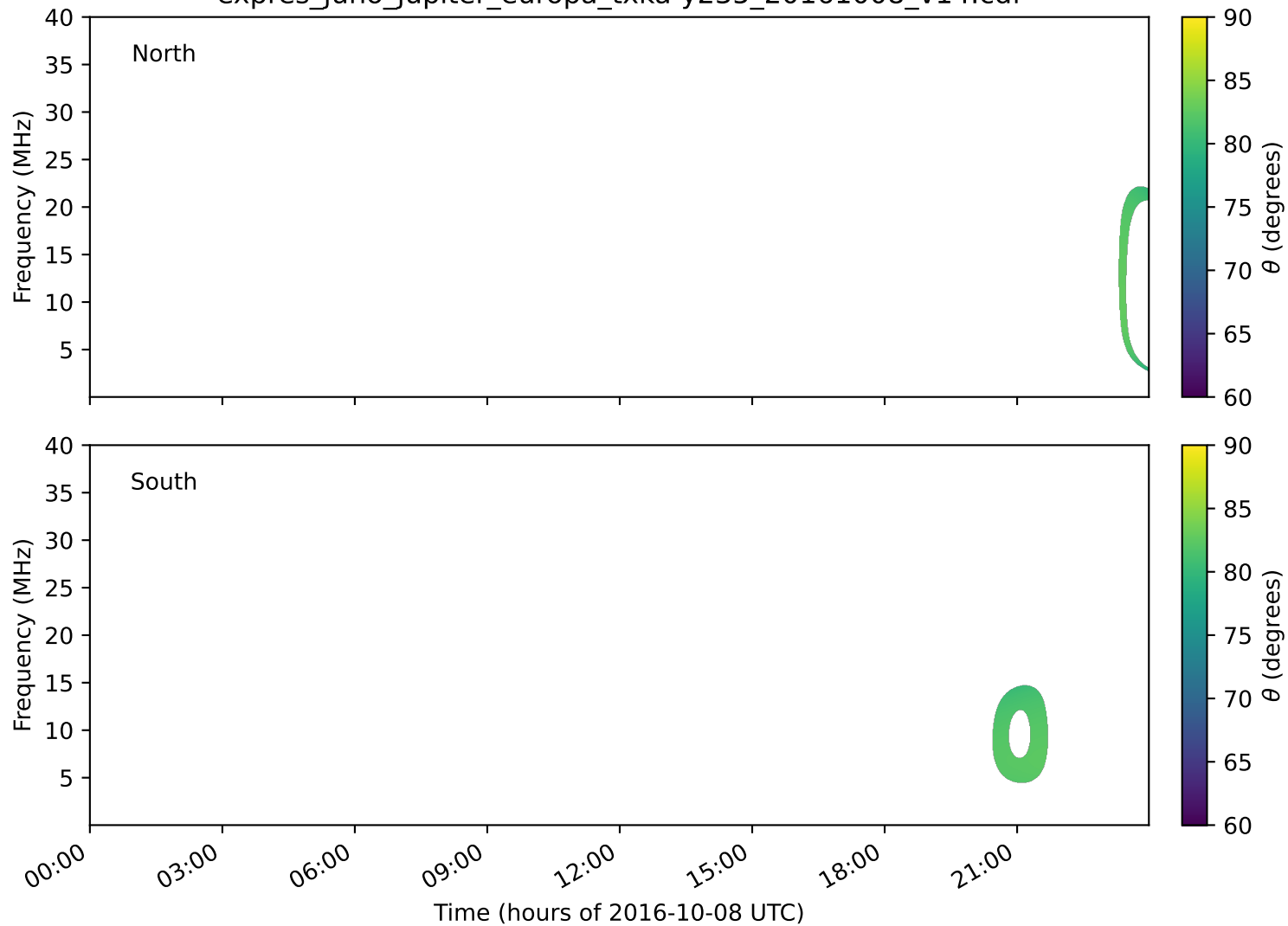
expres_juno_jupiter_europa_txka-y235_20161008_v14.cdf
