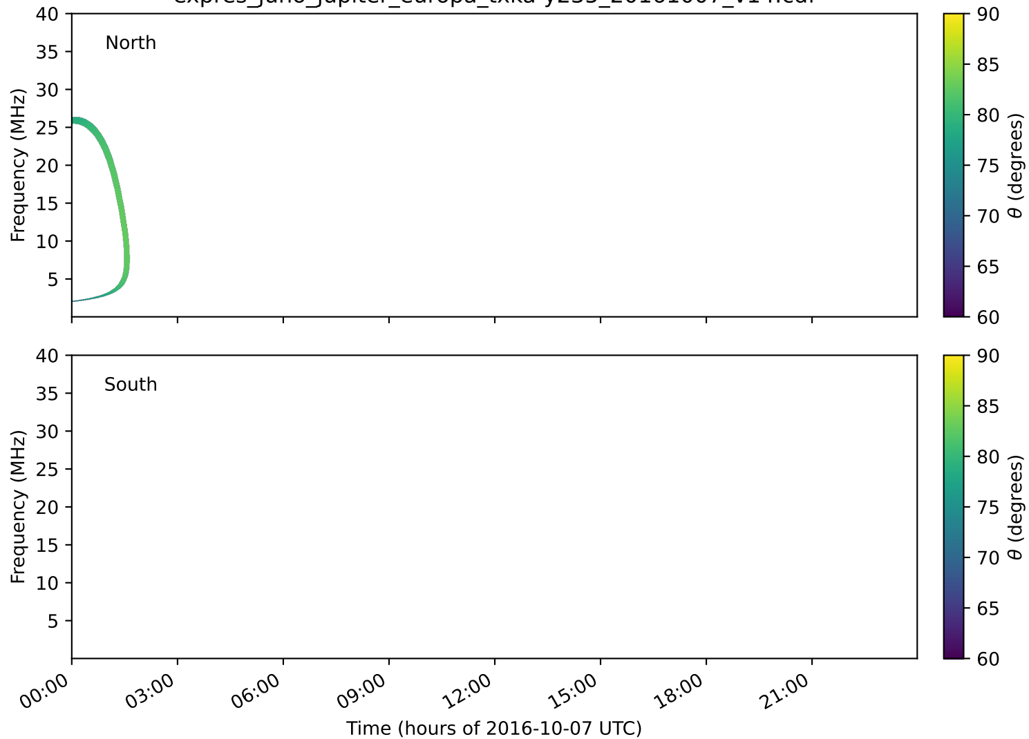
expres_juno_jupiter_europa_txka-y235_20161007_v14.cdf
