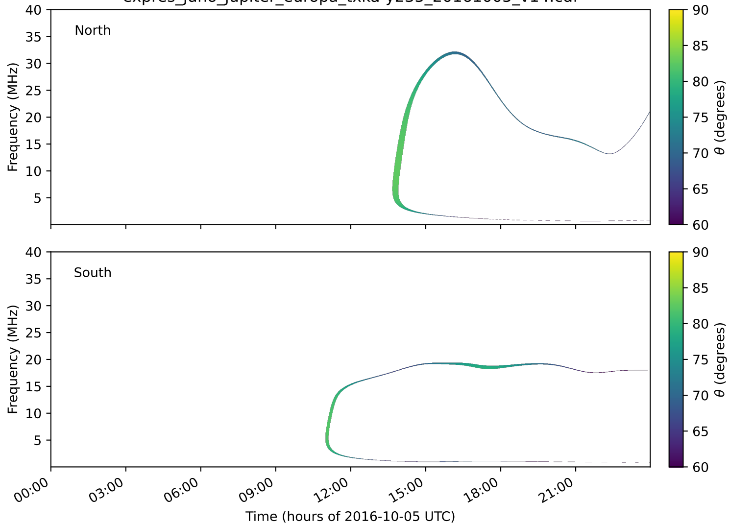
expres_juno_jupiter_europa_txka-y235_20161005_v14.cdf
