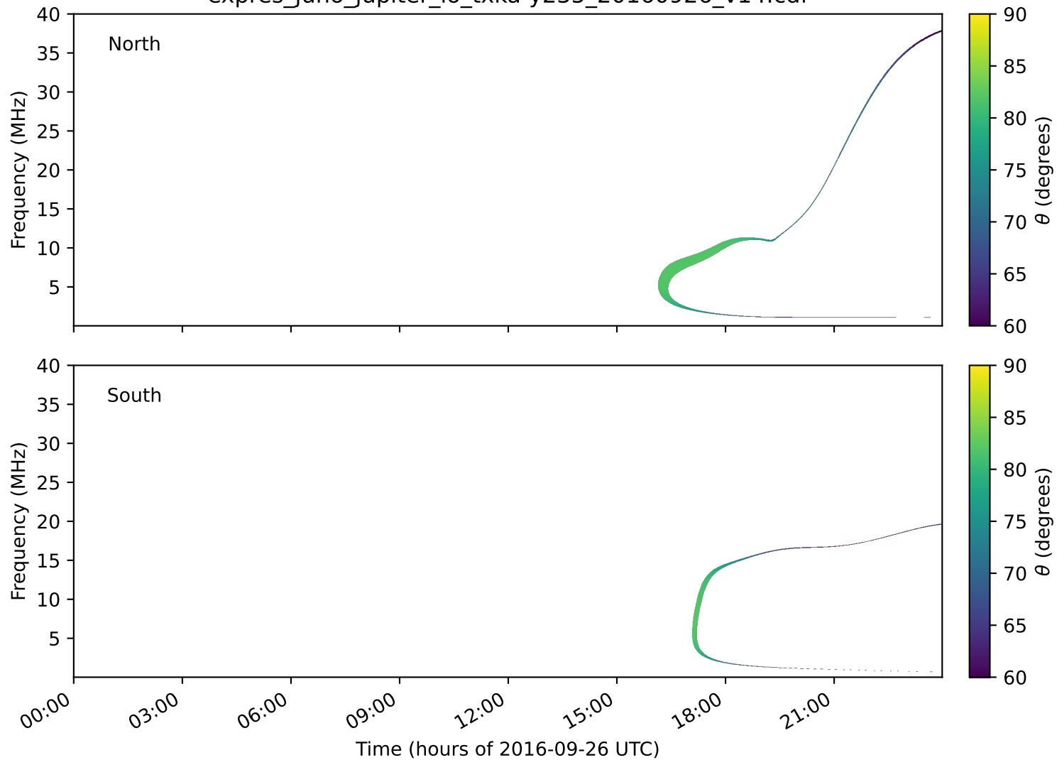
expres_juno_jupiter_io_txka-y235_20160926_v14.cdf
