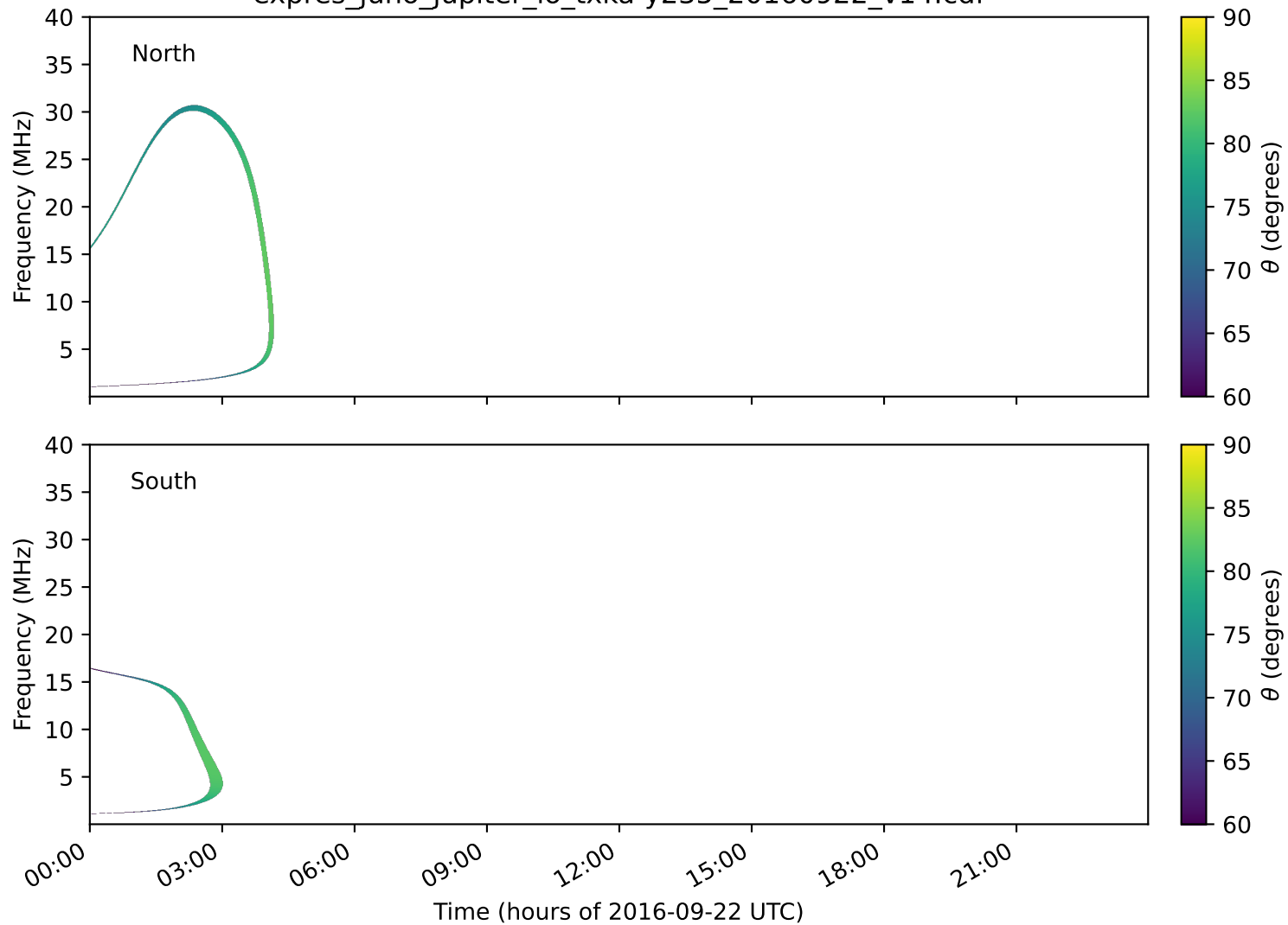
expres_juno_jupiter_io_txka-y235_20160922_v14.cdf
