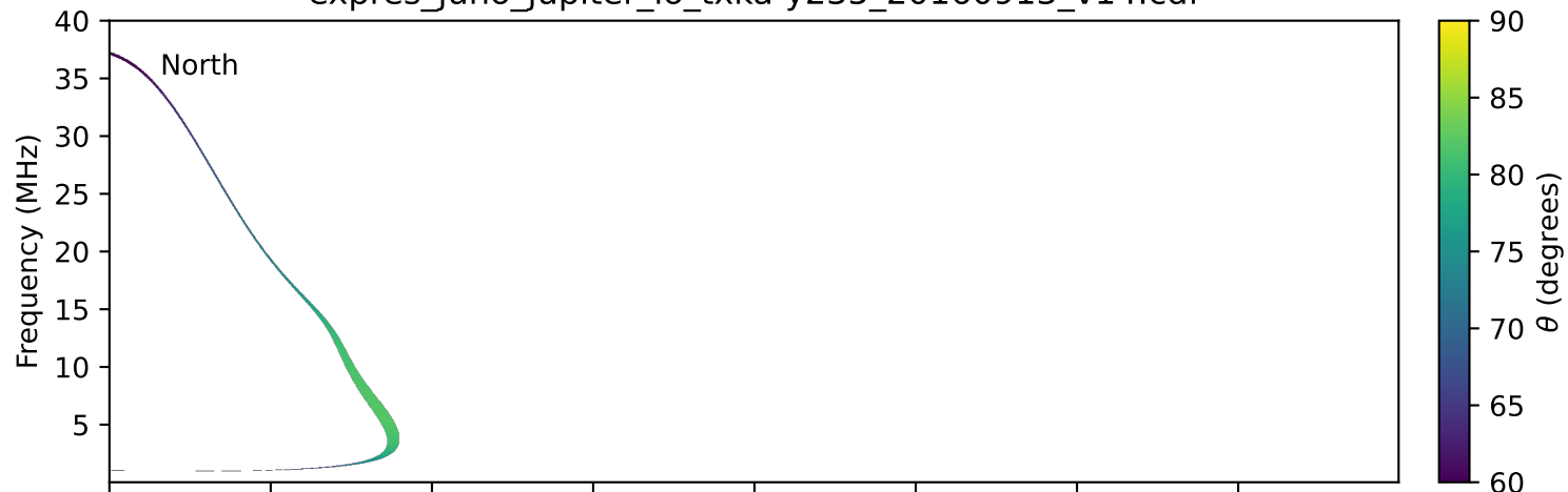
expres_juno_jupiter_io_txka-y235_20160913_v14.cdf
