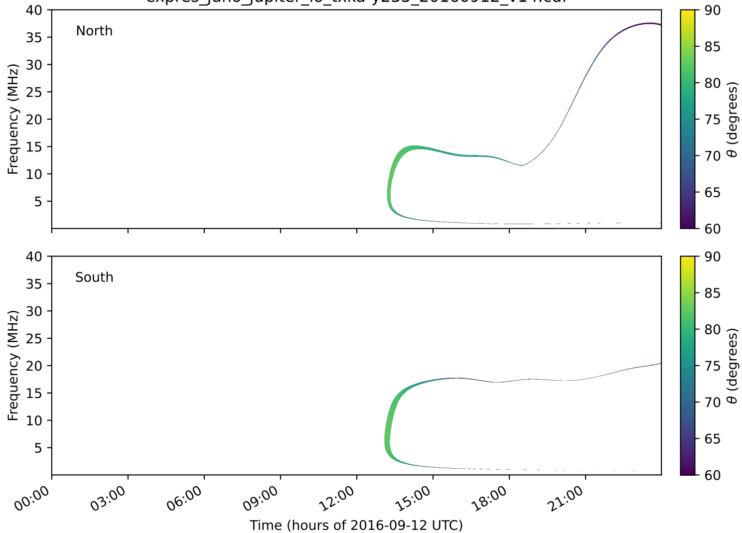
expres_juno_jupiter_io_txka-y235_20160912_v14.cdf
