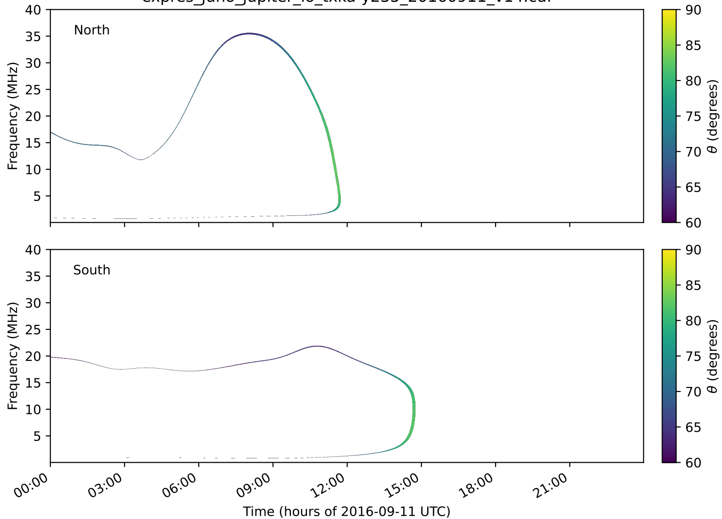
expres_juno_jupiter_io_txka-y235_20160911_v14.cdf
