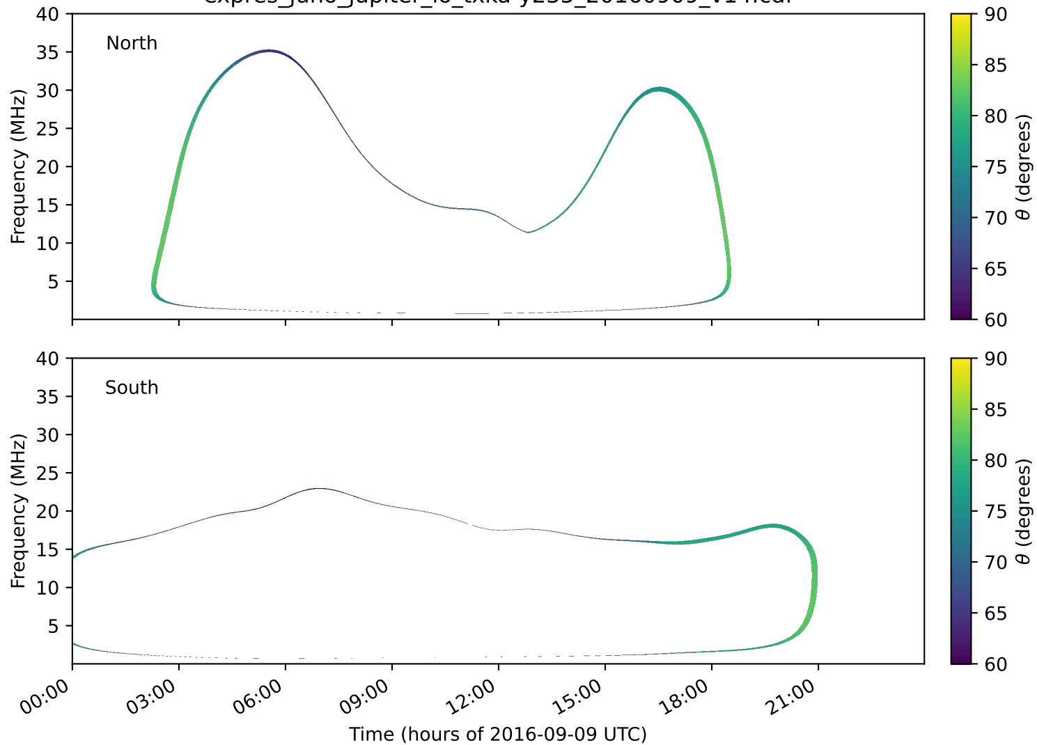
expres_juno_jupiter_io_txka-y235_20160909_v14.cdf
