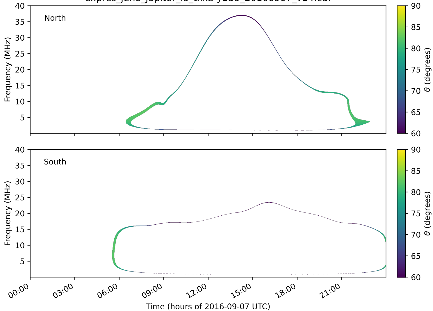
expres_juno_jupiter_io_txka-y235_20160907_v14.cdf
