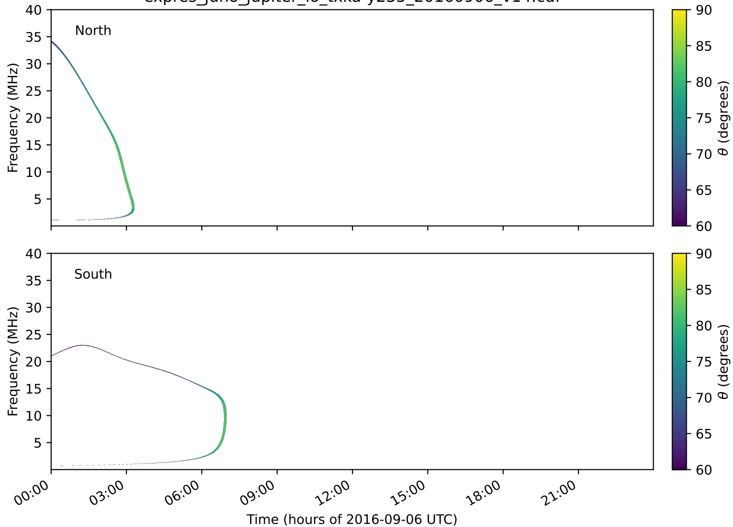
expres_juno_jupiter_io_txka-y235_20160906_v14.cdf
