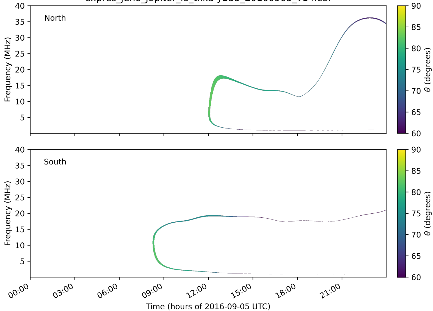
expres_juno_jupiter_io_txka-y235_20160905_v14.cdf
