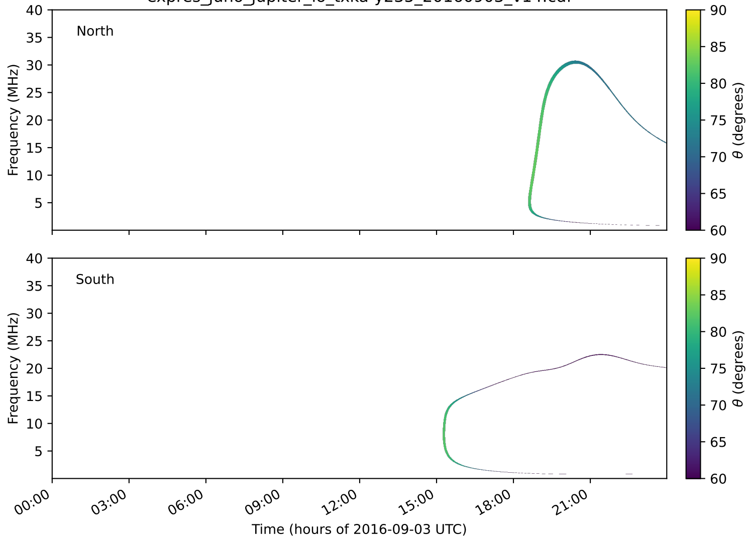
expres_juno_jupiter_io_txka-y235_20160903_v14.cdf
