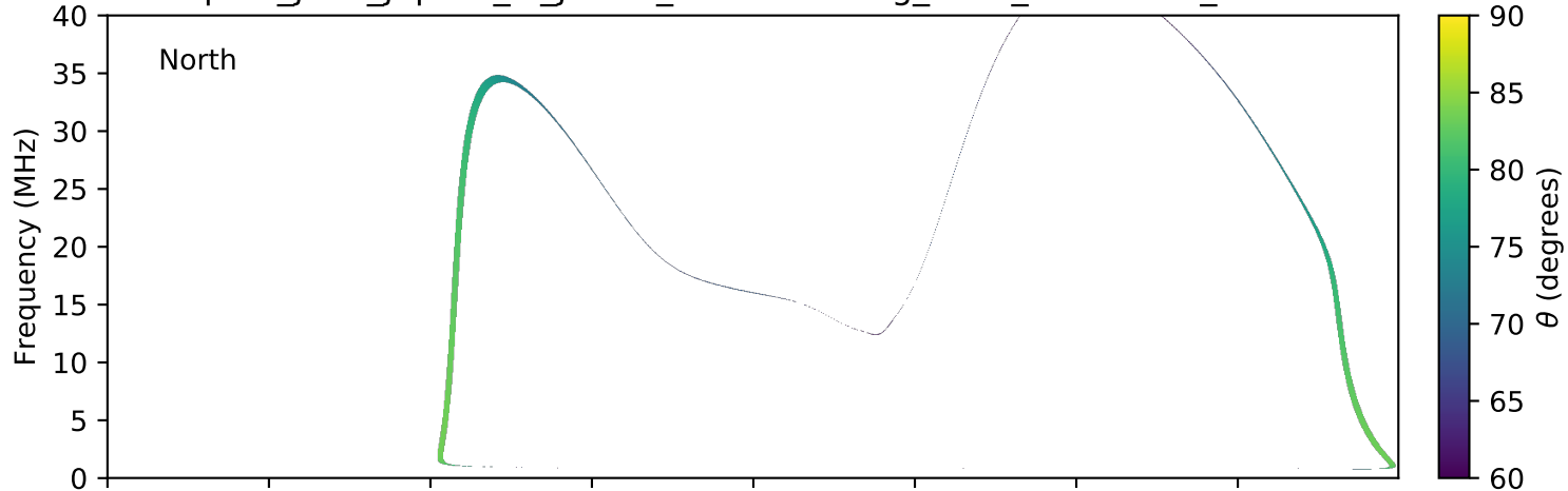
expres_juno_jupiter_io_jrm09_lossc-wid1deg_3kev_20160930_v01.cdf
