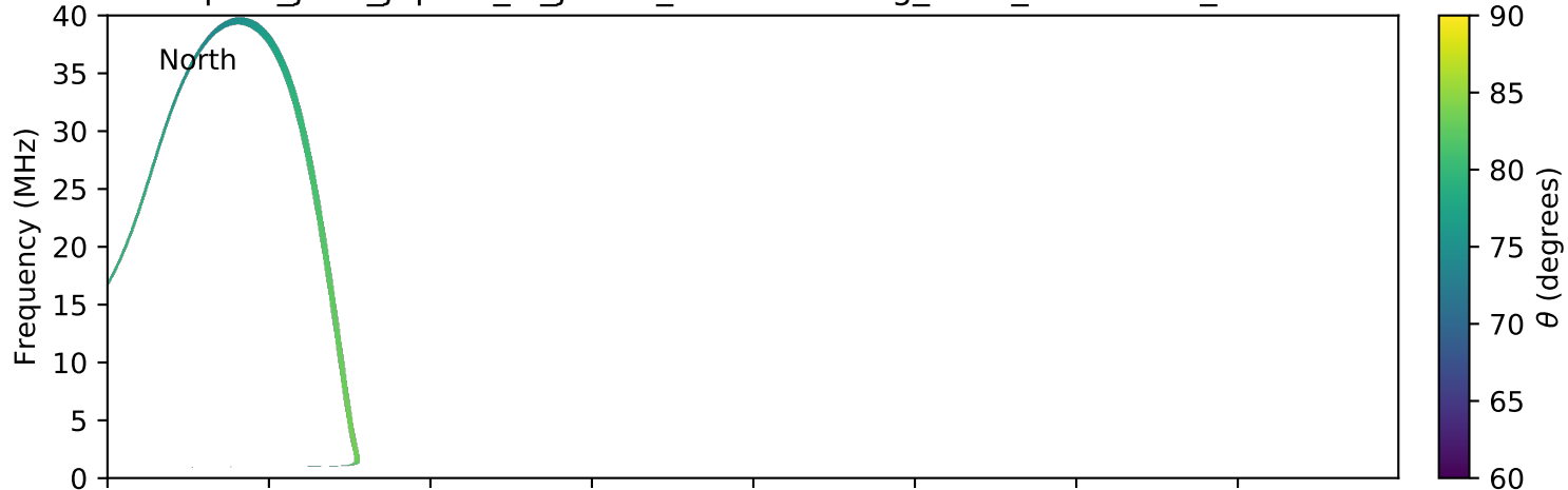
expres_juno_jupiter_io_jrm09_lossc-wid1deg_3kev_20160922_v01.cdf
