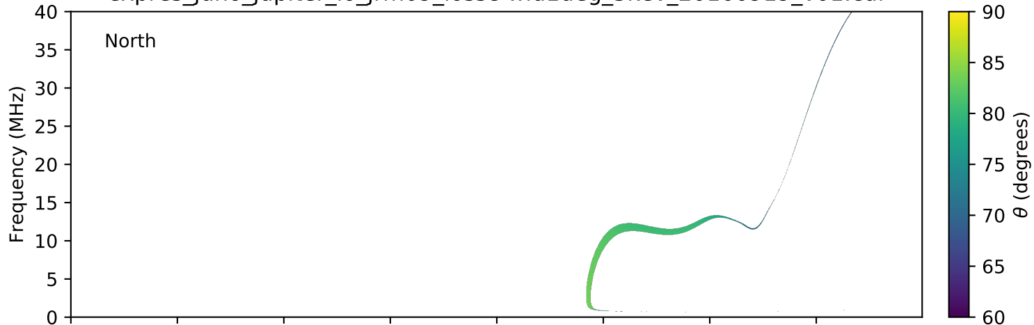
expres_juno_jupiter_io_jrm09_lossc-wid1deg_3kev_20160919_v01.cdf
