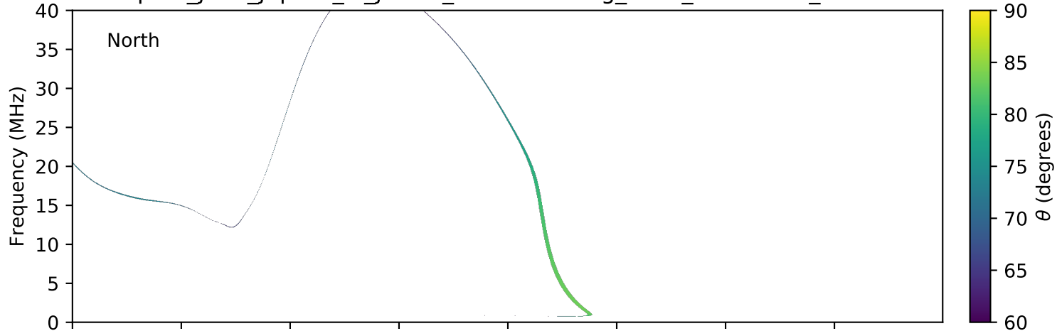
expres_juno_jupiter_io_jrm09_lossc-wid1deg_3kev_20160918_v01.cdf
