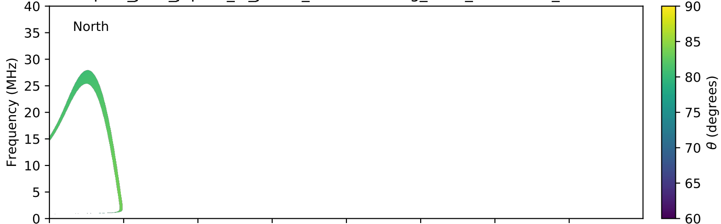
expres_juno_jupiter_io_jrm09_lossc-wid1deg_3kev_20160915_v01.cdf
